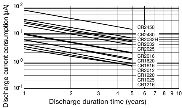
Fig. 1 Relationship between Discharge Current Consumption and Duration Time
